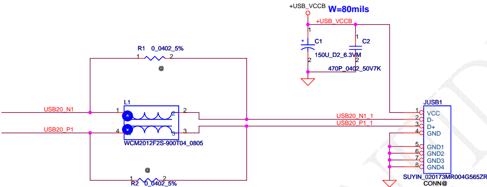
USB CONN1.
