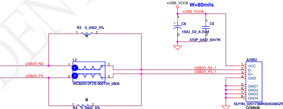
USB CONN2.
